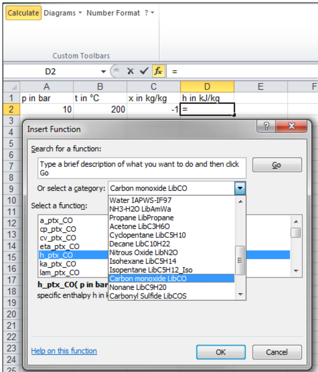
Figure 2.14: Choice of library and function name
