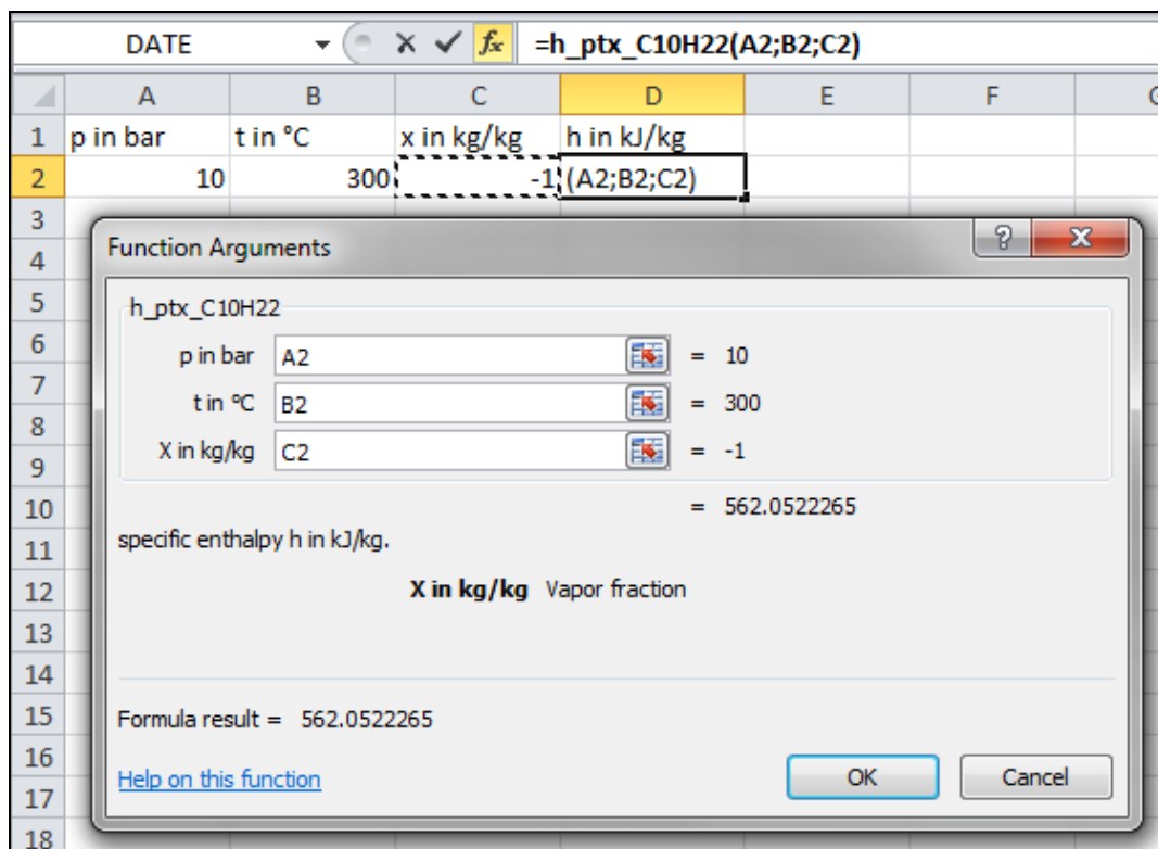
Figure 2.16: Input menu showing the result
