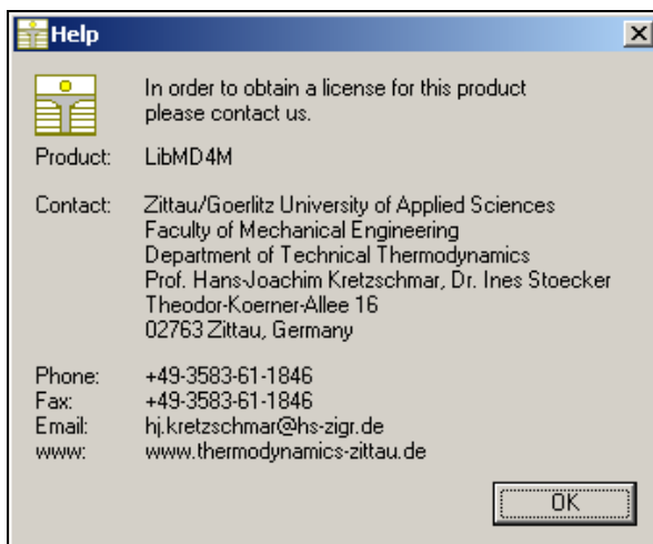
Figure 2.3: "Help" window
